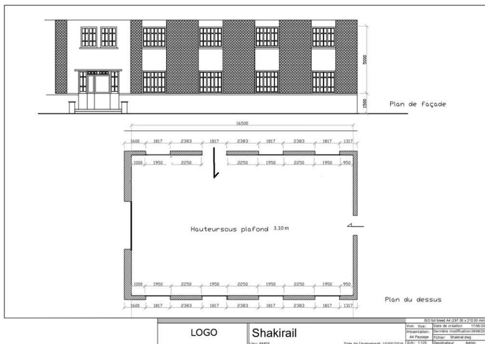
Plan grande salle - Shakirail
